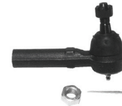
CR1012 Outer Tie Rod End (Ø12.4*Ø15.2/M14*1.5)
