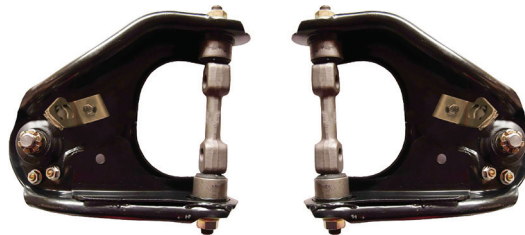
IS1716 Upper Control Arm 1989-1997
